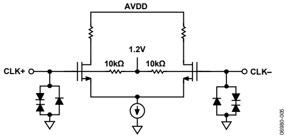
Figure 35. CLK± Inputs
