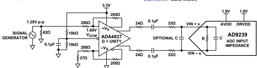
Figure 45. Differential Amplifier Configuration for AC-Coupled Baseband Applications
