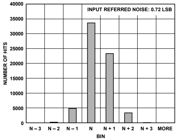
Figure 29. Input-Referred Noise Histogram, f_{SAMPLE} = 170 \text{ MSPS}
