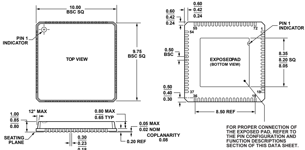
Figure 80. 72-Lead Lead Frame Chip Scale Package [LFCSP_VQ] 10 mm × 10 mm Body, Very Thin Quad (CP-72-3) Dimensions shown in millimeters
