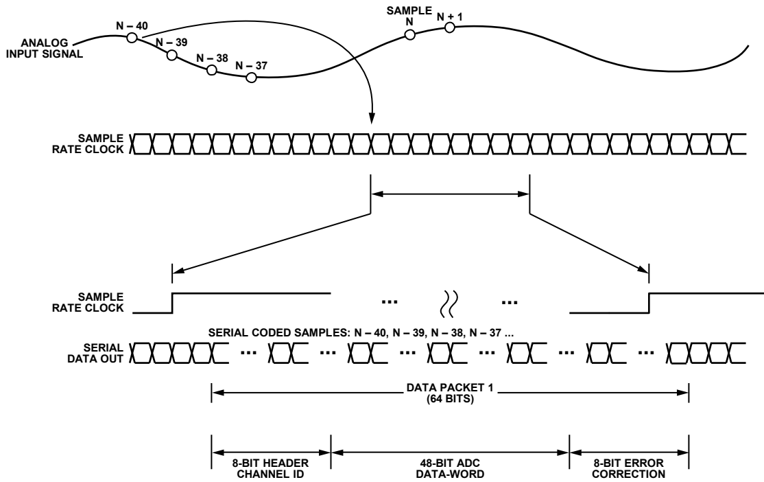
Figure 2. Timing Diagram
